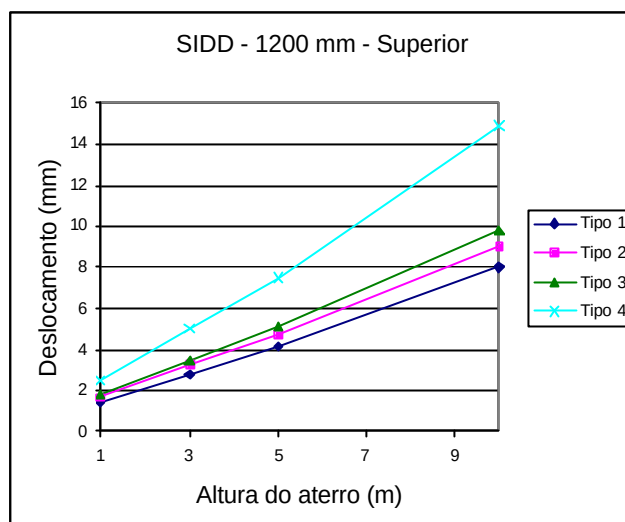
Figura 5.10 – Deslocamento vertical no topo ( d_i = 1200 mm)
