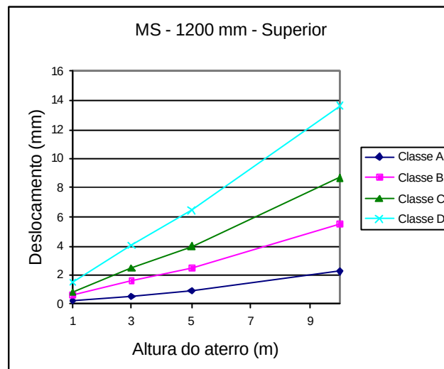
Figura 5.19 – Deslocamento vertical no topo ( d_i = 1200 mm)
